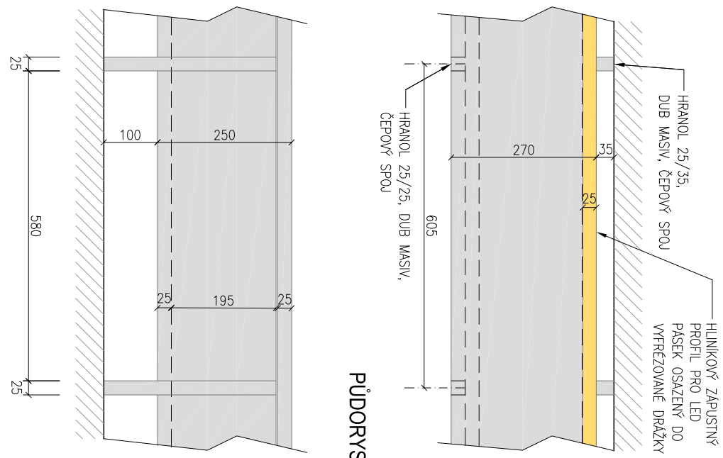
DETAIL 01 - ENERGOKANÁLEK 270x250 mm
