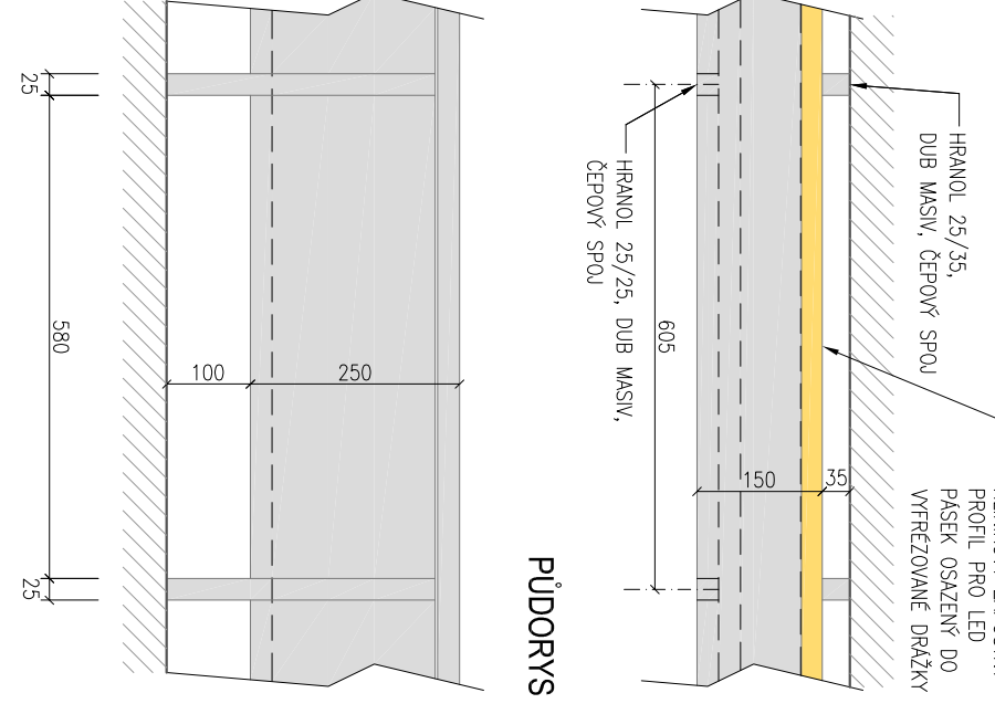
DETAIL 03 - ENERGOKANÁLEK 150x250 mm
