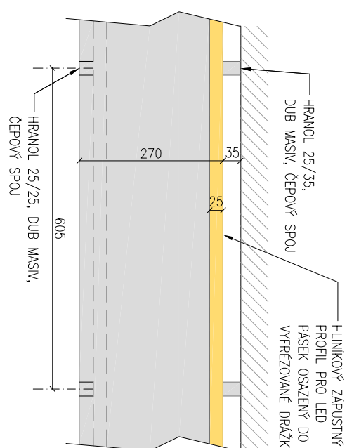
DETAIL 01 - ENERGOKANÁLEK 270x250 mm
