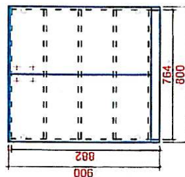
AT 383 60 hloubka 598 mm 3x poloh. police
